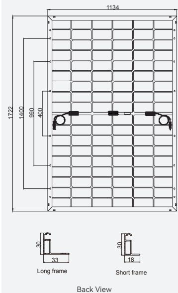
Back View
